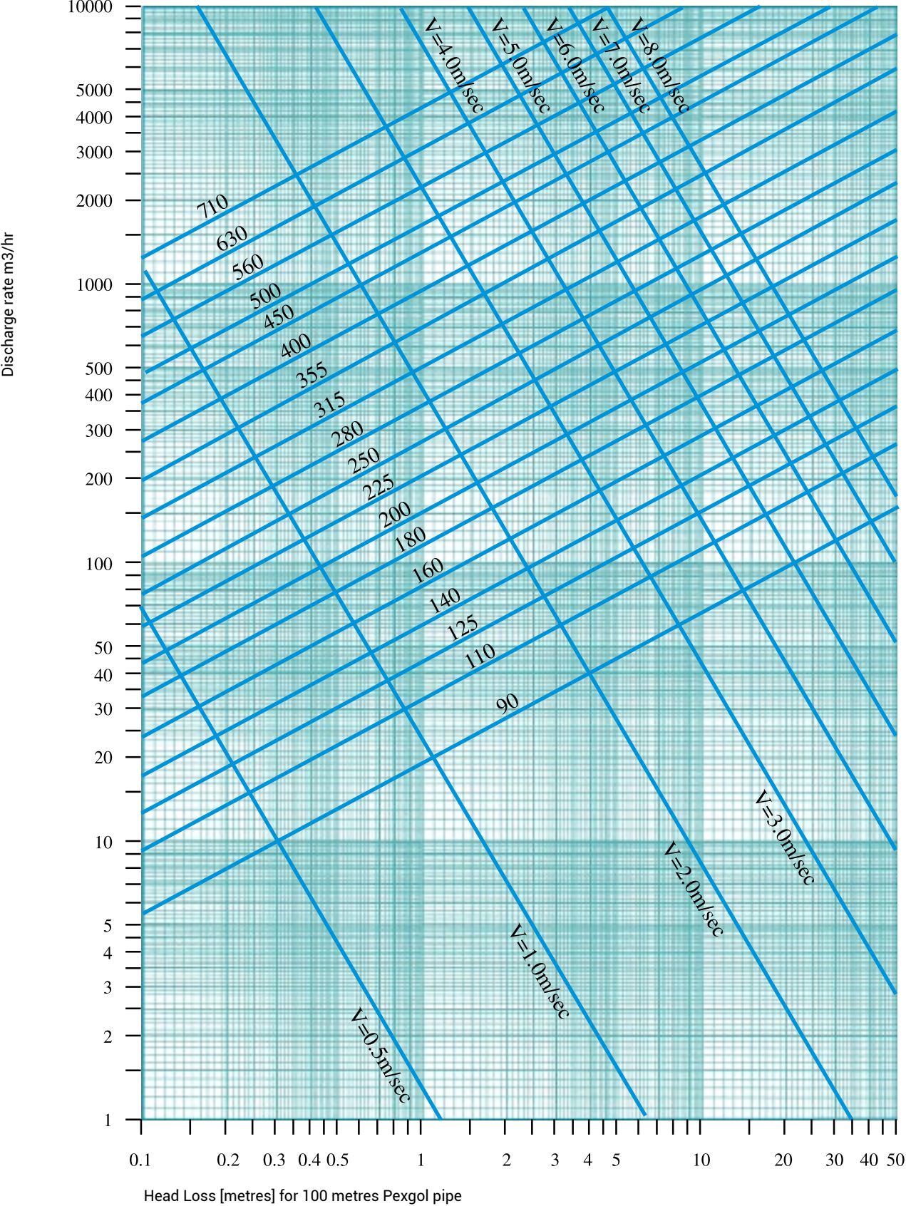
Chart 15.1: Class 6 (SDR 26)
